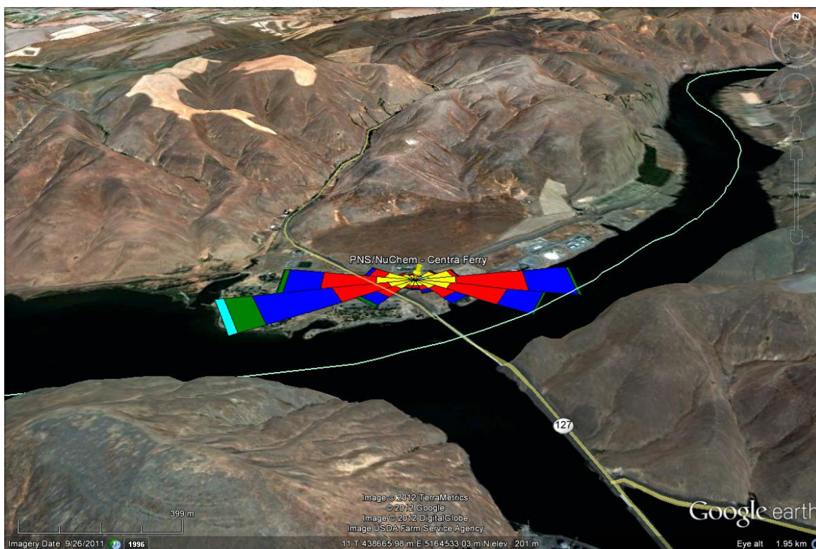
Diagram 1: Wind Rose Created with Pullman/Moscow Airport Data (2007 – 2011) at NuChem, Central Ferry
