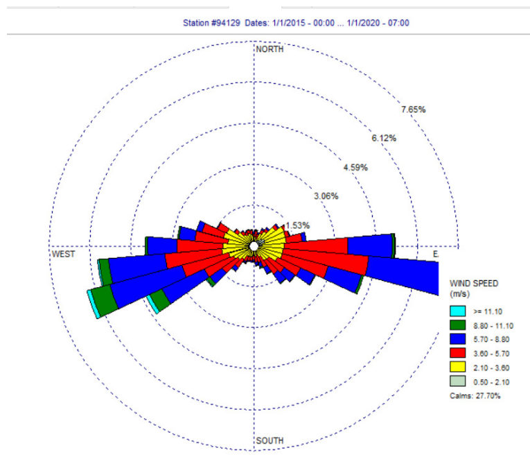
Diagram 2: 5-Yr Wind Rose
