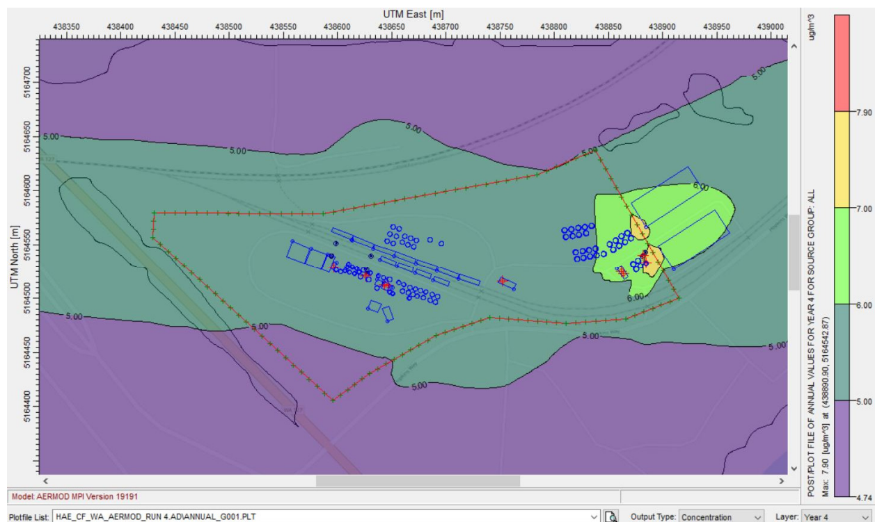
Diagram 9: First High Annual Average Concentration + Background (Year 4 – Highest Year)
