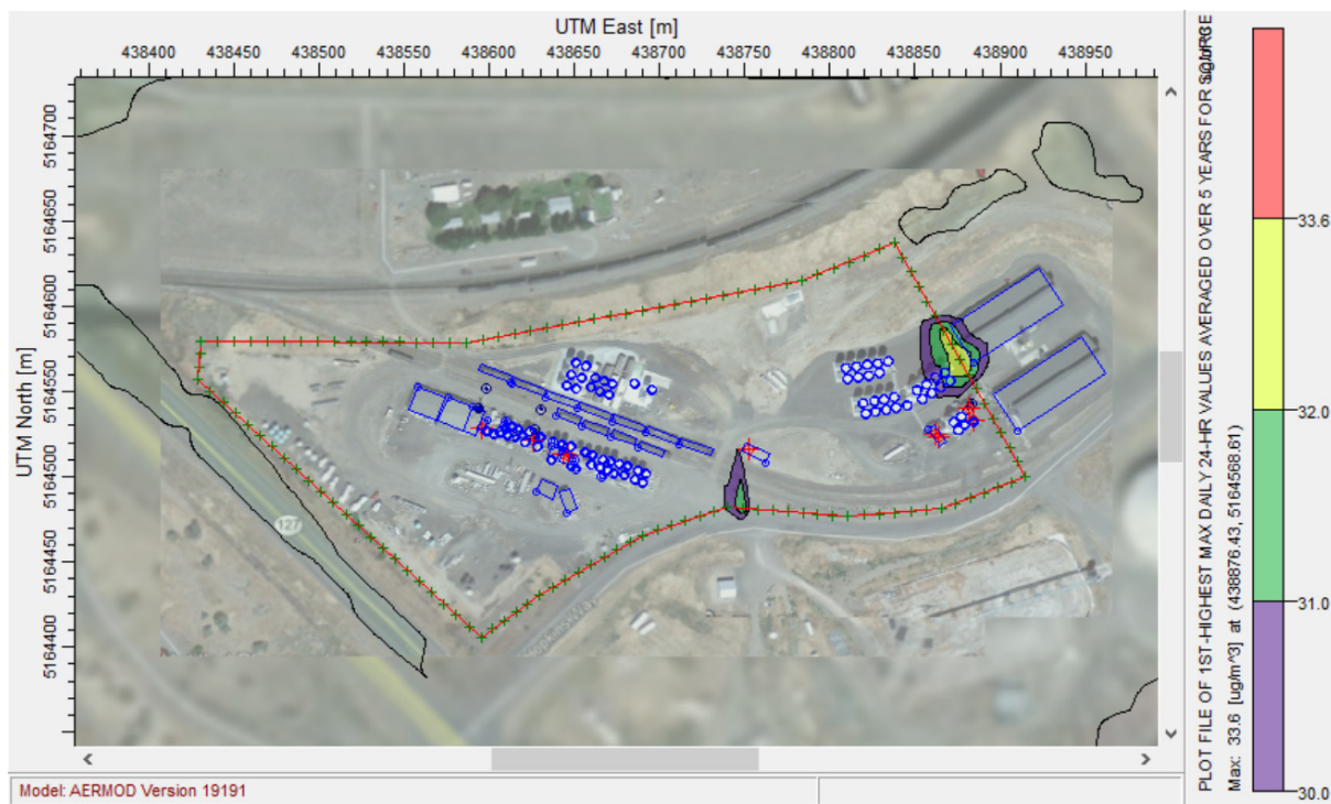
Diagram 8: 5-Yr Average of the First High PM2.5 24-hour Average Concentrations
