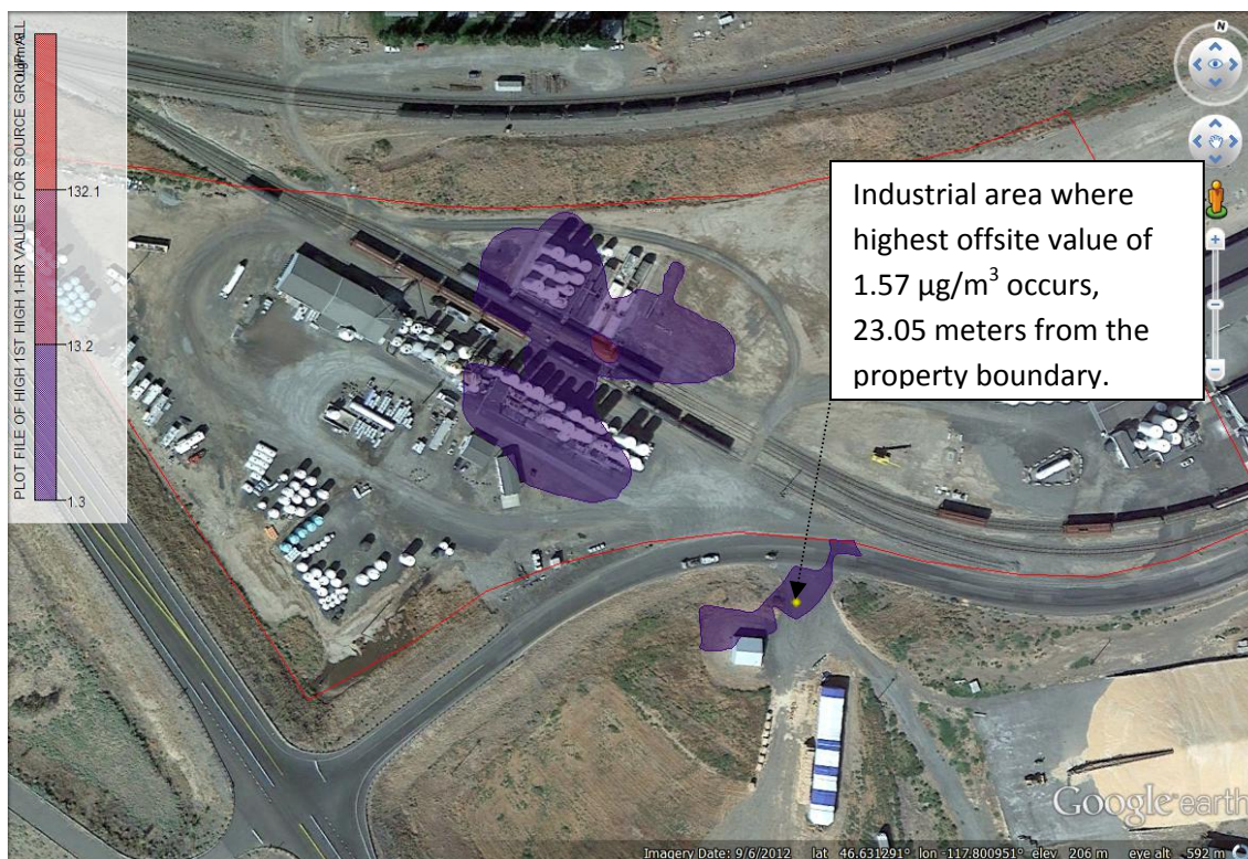
Diagram 6: 1 st High – 1 Hour Concentrations of Fluoride (Comparison to NRC Value of 1,321 \mu\text{g}/\text{m}^3 )
