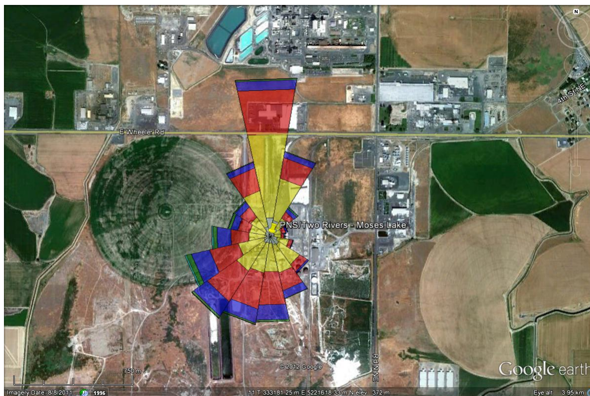
Diagram 2: Wind Rose Created with Grant County Airport Data (2007 – 2011) at Two Rivers, Moses Lake
