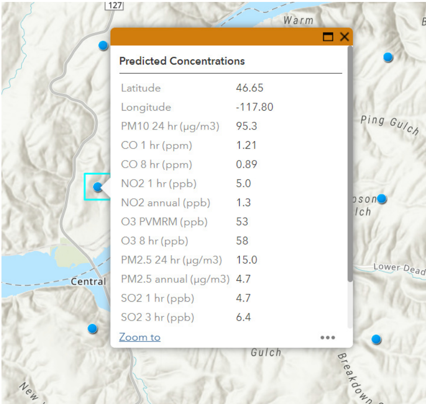
Diagram 6: Background Concentration in Area
