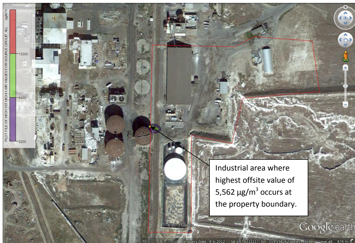
Diagram 14: 1 st High – 1 Hour Concentrations of Ammonia, Overview of Site
