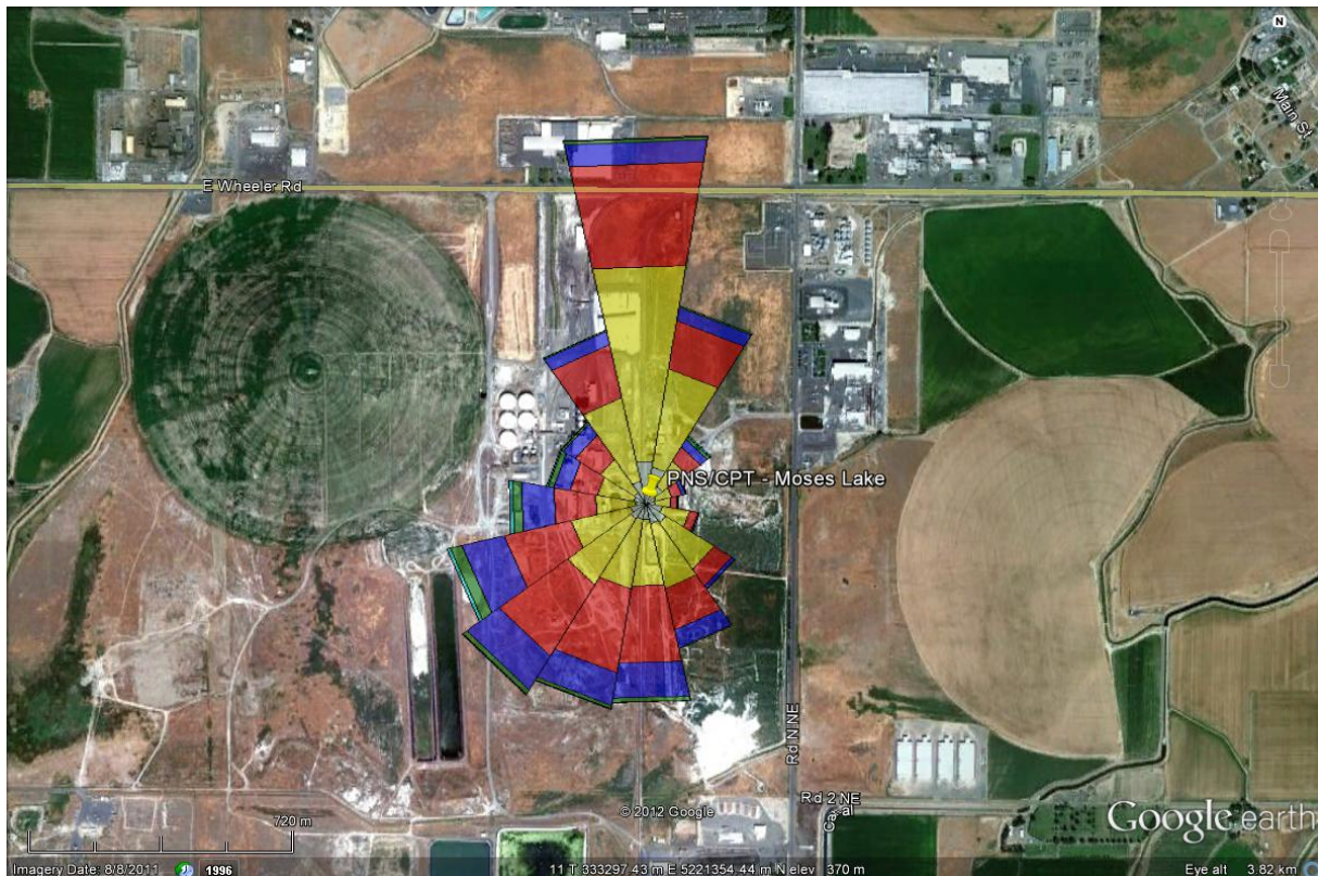
Diagram 3: Wind Rose Created with Grant County Airport Data (2007 – 2011) at CPS, Moses Lake
