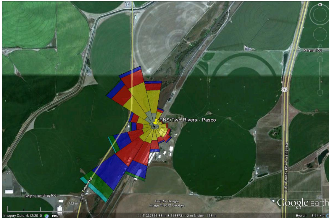
Diagram 4: Wind Rose Created with Tri-Cities Airport Data (2007 – 2011) at Two Rivers, Pasco
