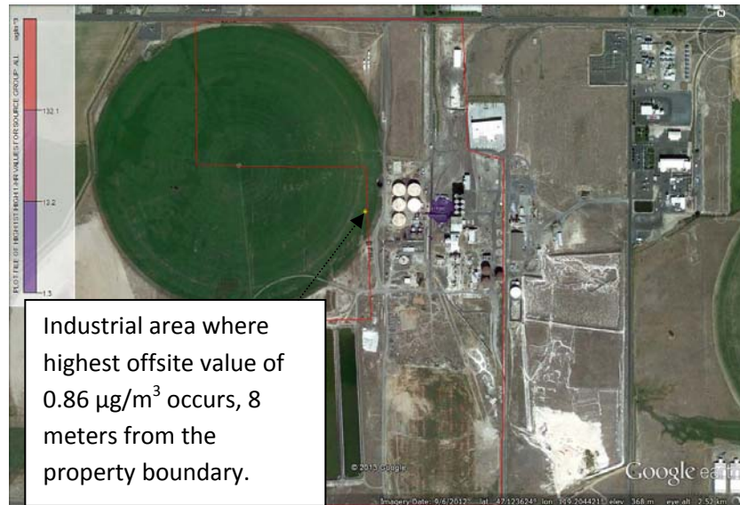
Diagram 10: 1 st High – 1 Hour Concentrations of Ammonia (Comparison to Cal OEHHA Value of 3,200 \mu\text{g}/\text{m}^3 )
