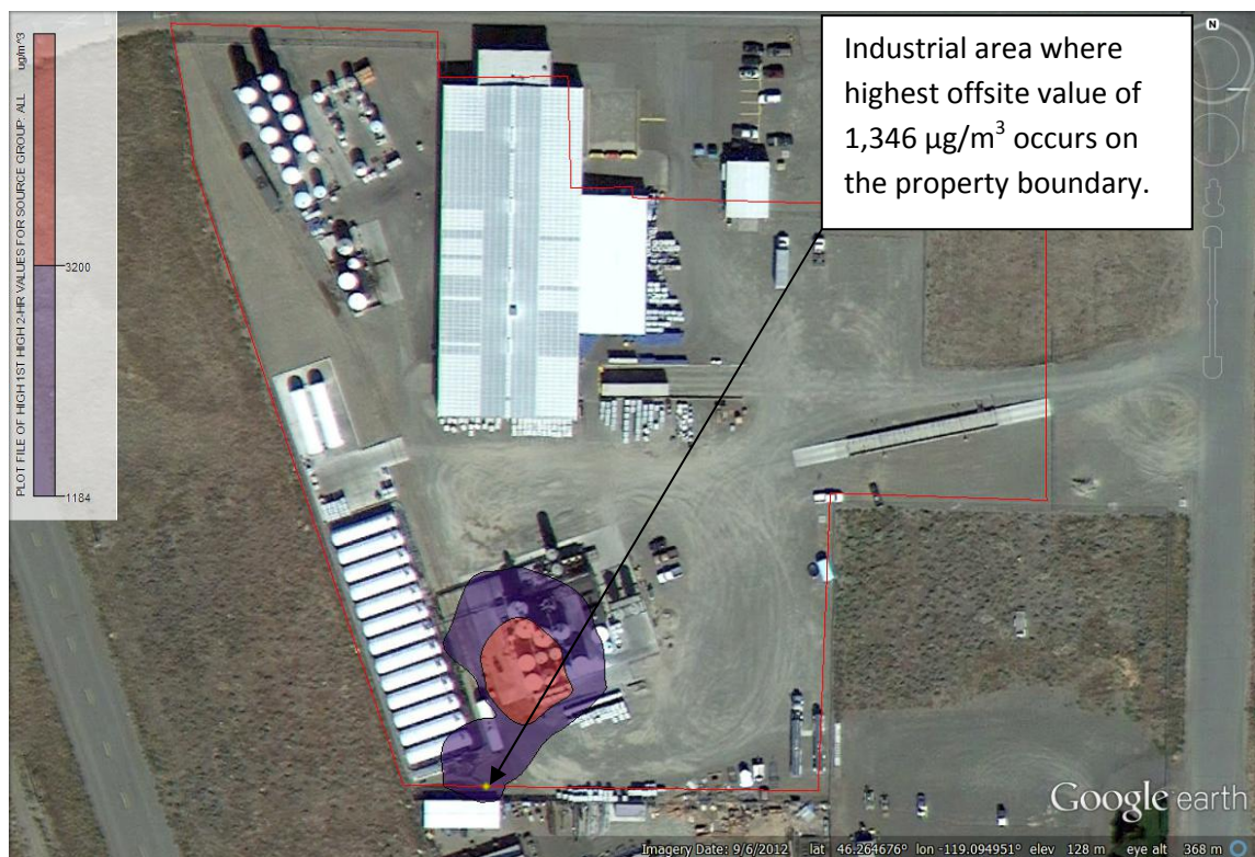
Diagram 21: 1 st High – 2 Hour Concentrations of Ammonia (Comparison to ATSDR Value of 1,184 \mu\text{g}/\text{m}^3 )
