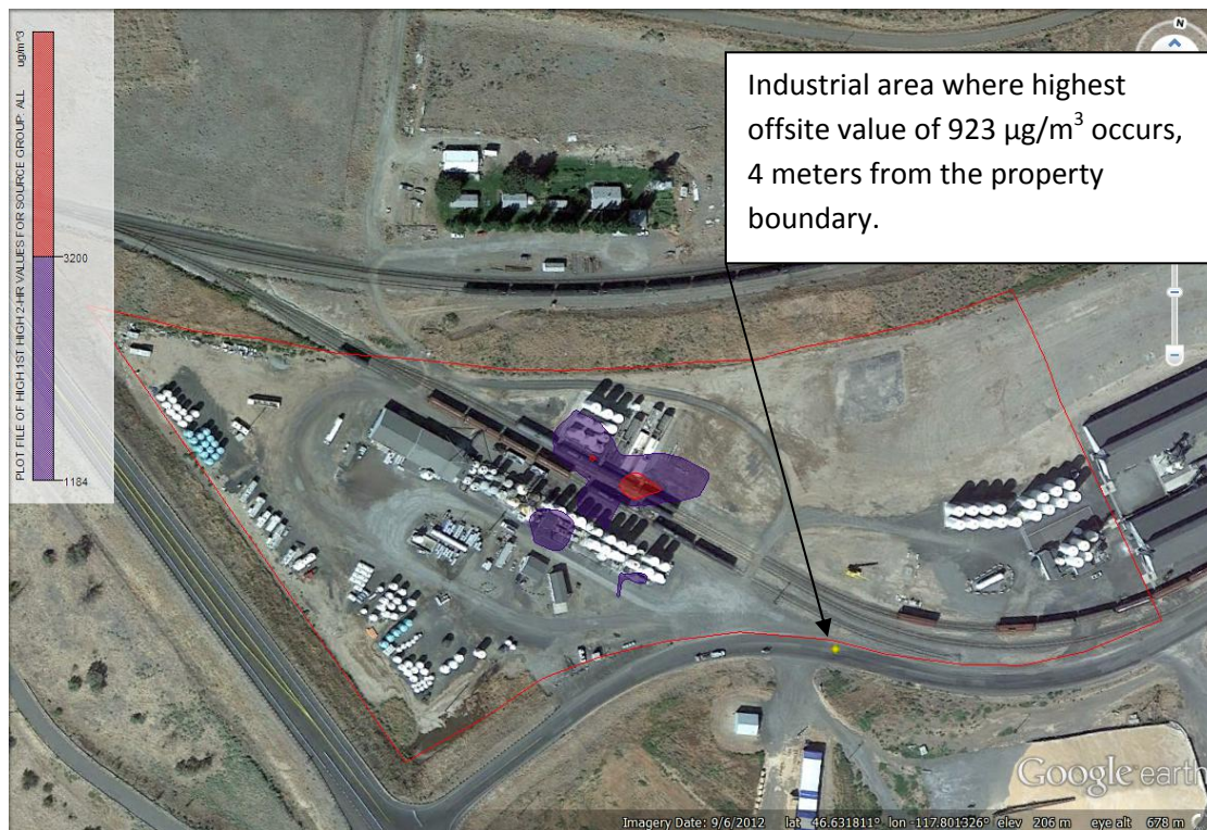
Diagram 8: 1 st High – 2 Hour Concentrations of Ammonia (Comparison to ATSDR Value of 1,184 \mu\text{g}/\text{m}^3 )
