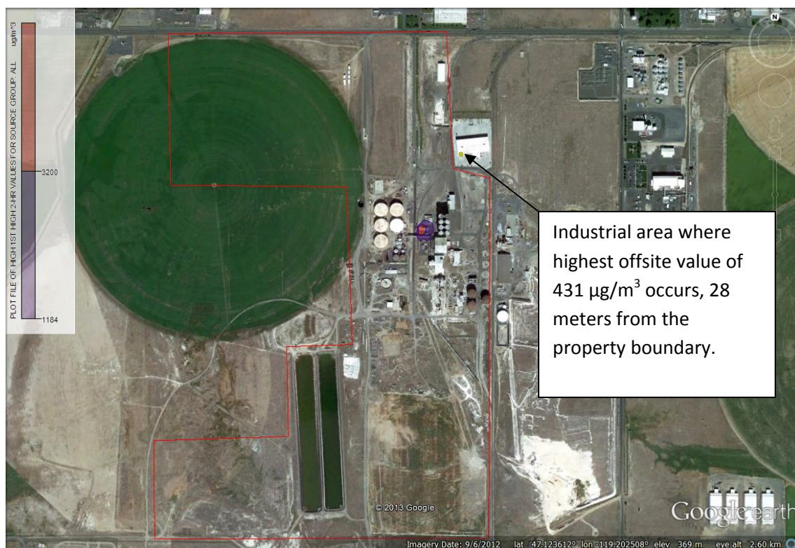
Diagram 11: 1 st High – 2 Hour Concentrations of Ammonia (Comparison to ATSDR Value of 1,184 \mu\text{g}/\text{m}^3 )
