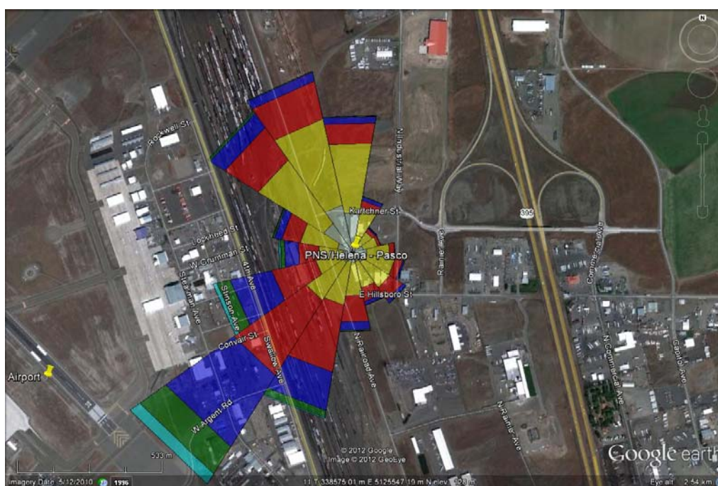
Diagram 5: Wind Rose Created with Tri-Cities Airport Data (2007 – 2011) at Helena, Pasco
