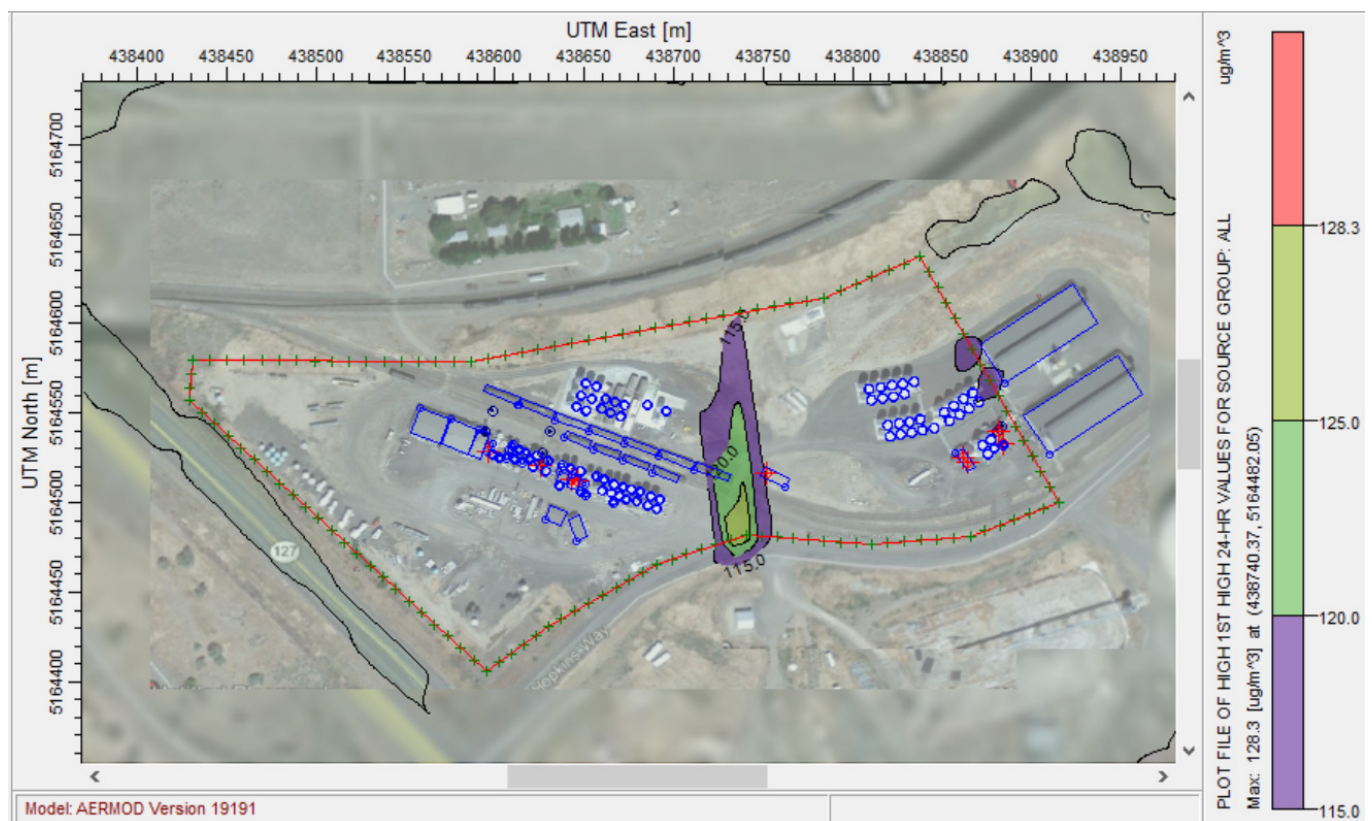
Diagram 7: First High PM 10 Concentrations + Background Over All 5-Yrs of Met Data
