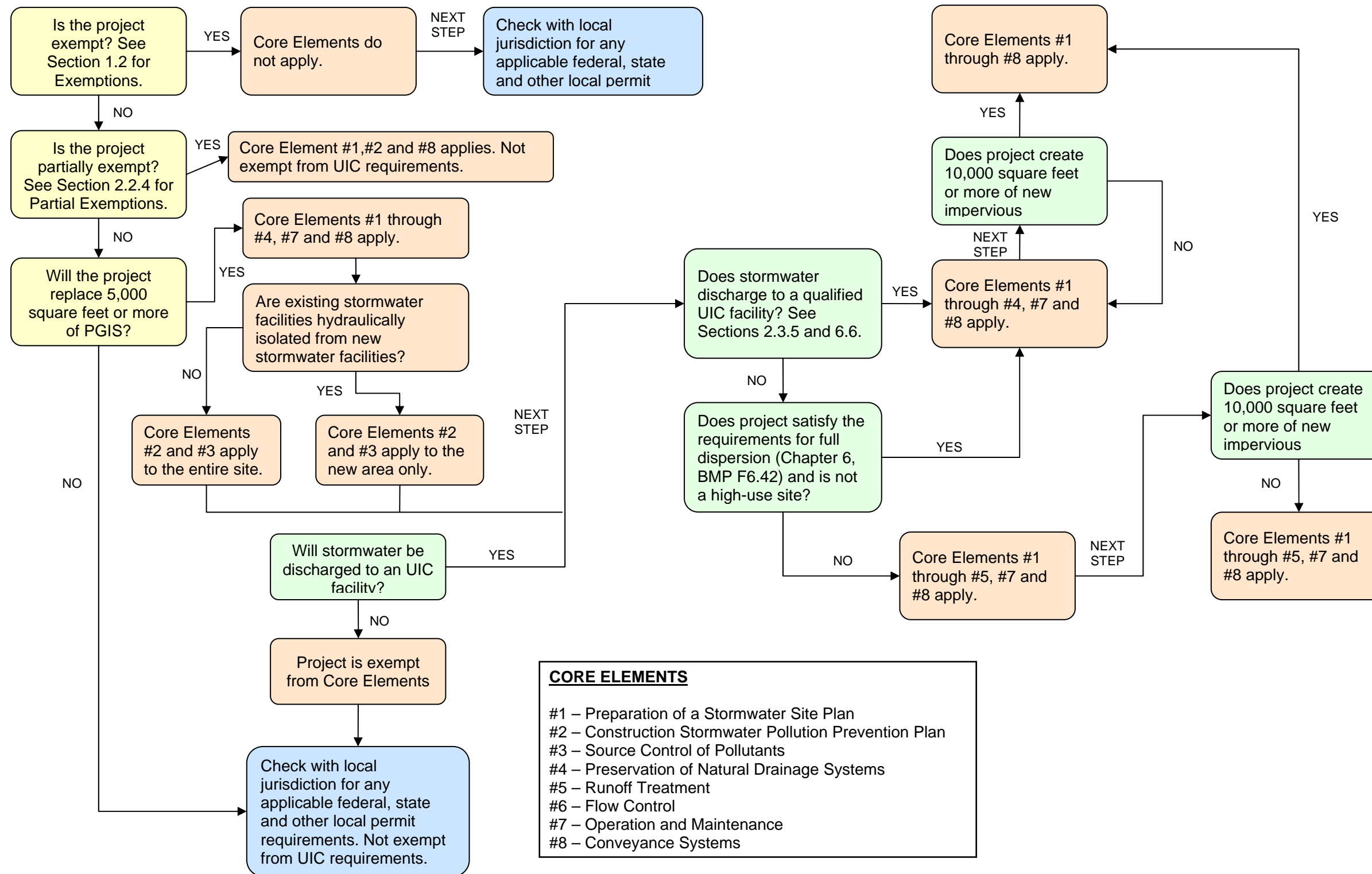
FIGURE 2.2 - REDEVELOPMENT CORE ELEMENT FLOW CHART
